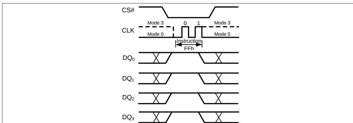
Figure 63 Disable QPI Instruction (QPI Mode only)
