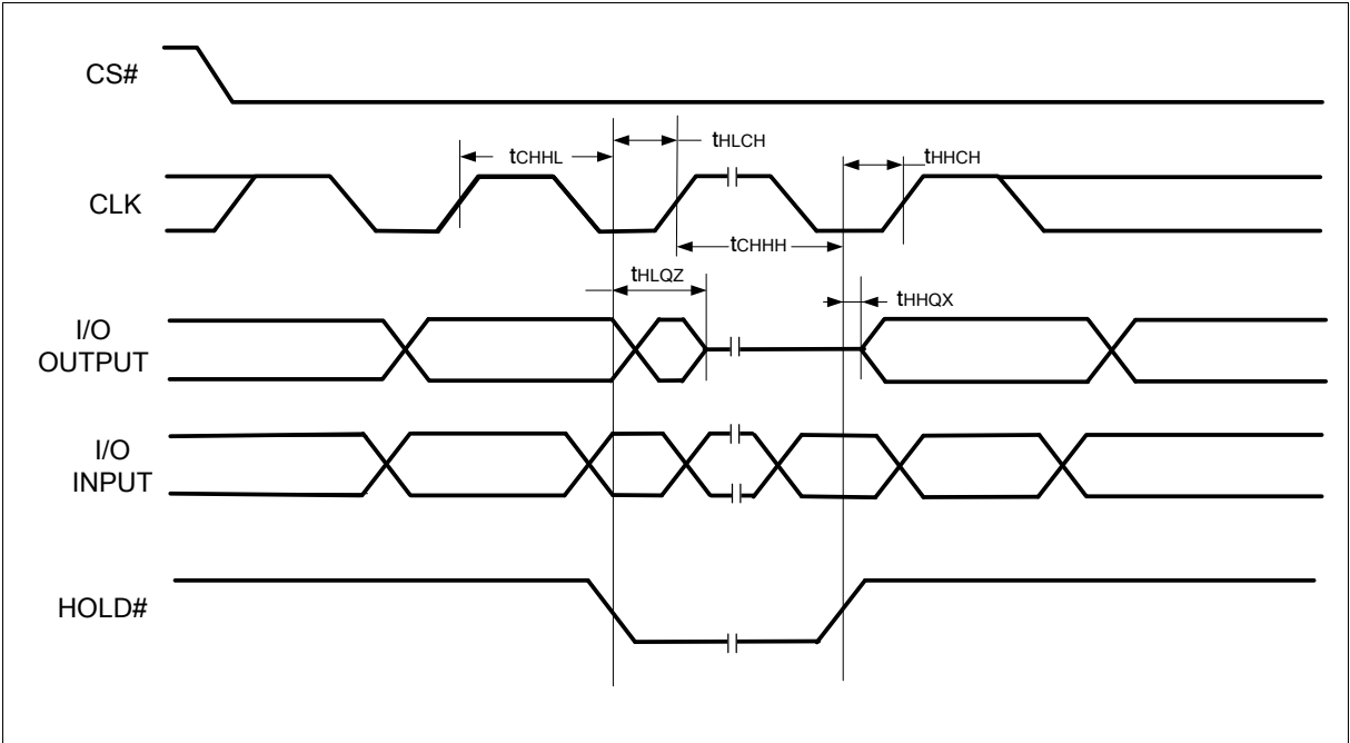
Figure 80 Hold Timing
