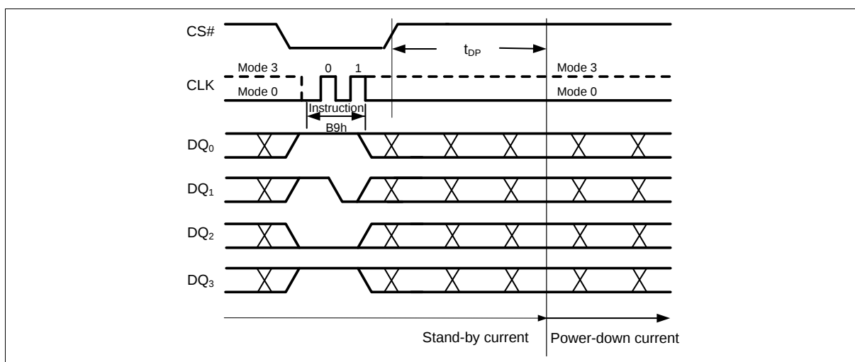
Figure 43 Deep Power-down Instruction (QPI Mode)
