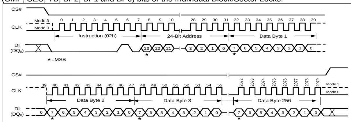
Figure 28 Page Program Instruction (SPI Mode)
