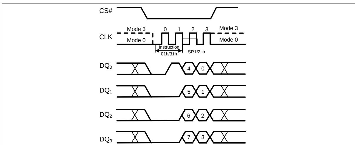
Figure 14 Write Status Register-1/2 Instruction (QPI Mode)
