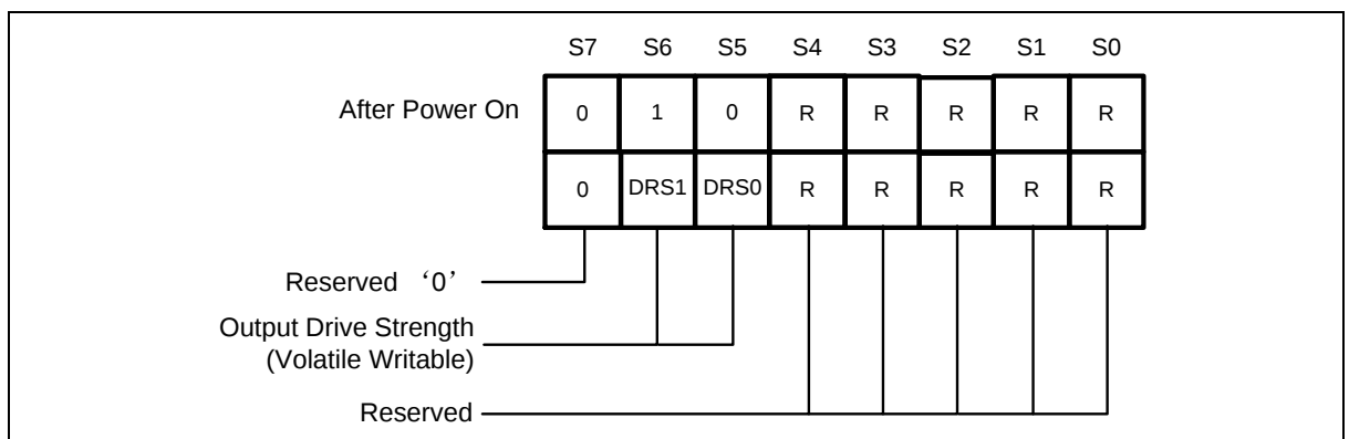
Figure 10 Status Register-4 (Address D0h)
