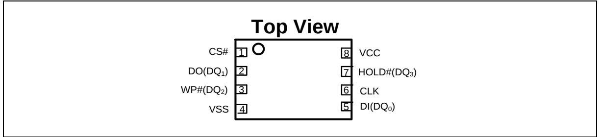
Figure 1 Pad Assignments, WSON8 8x6mm (TDFN8 8x6mm) & WSON8 5x6mm (TDFN8 5x6mm)
