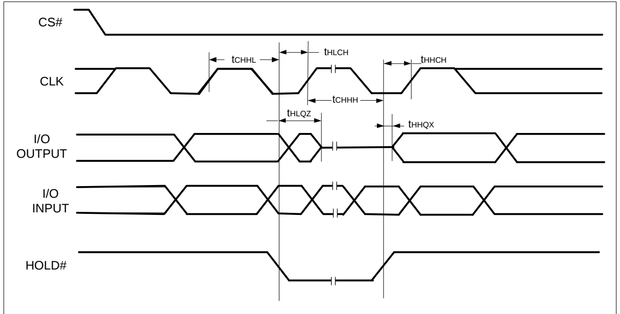
Figure 31 Hold Timing
