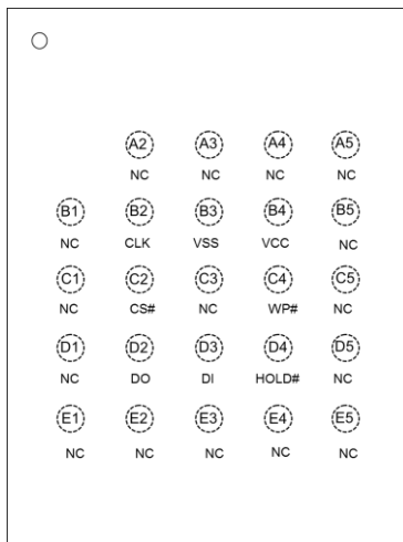
BGA24 8x6mm 5*5-1 Ball Array
