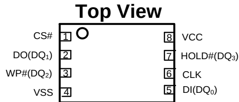
Figure 2 Pad Assignments
